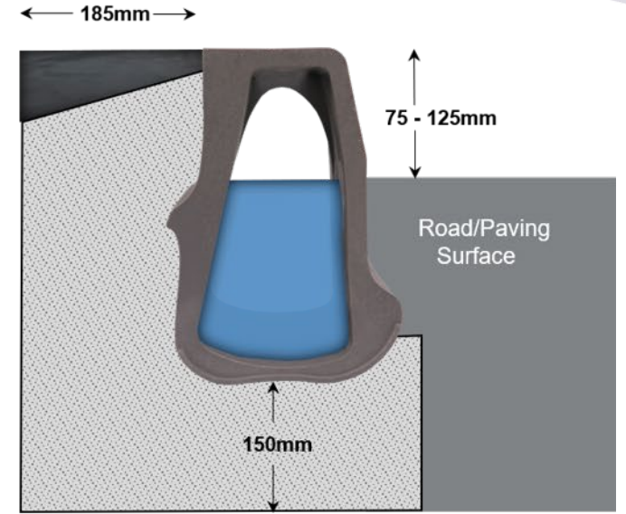
Typical Pavement-Backed Detail – Please view our Design & Installation Guide for more information.
